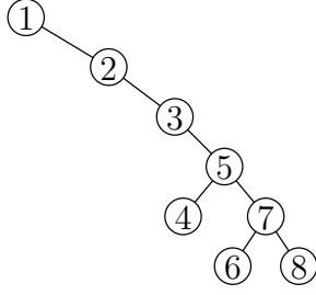
Fig. 1. T(\sigma) obtained from \sigma = (1, 2, 3, 5, 7, 4, 6, 8) . We have \text{height}(\sigma) = 6 .
