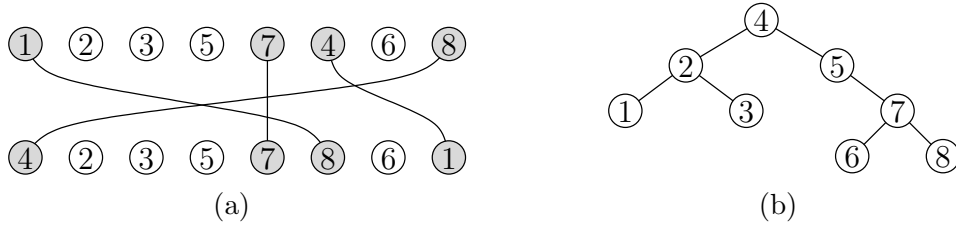
Fig. 2. A partial permutation. (a) Top: The sequence \sigma = (1, 2, 3, 5, 7, 4, 6, 8) with \mu = M_p^n = \{1, 5, 6, 8\} ; Figure 1 shows T(\sigma) . Bottom: The marked elements are randomly permuted. The result is \sigma' = \Pi(\sigma, \mu) = (4, 2, 3, 5, 7, 8, 6, 1) . (b) T(\sigma') with \text{height}(\sigma') = 4 .
