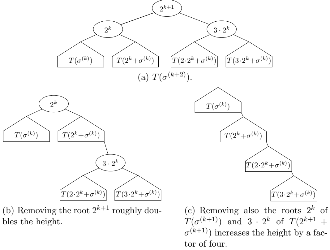
Fig. 4. Removing root elements increases the height and the number of left-to-right maxima.
