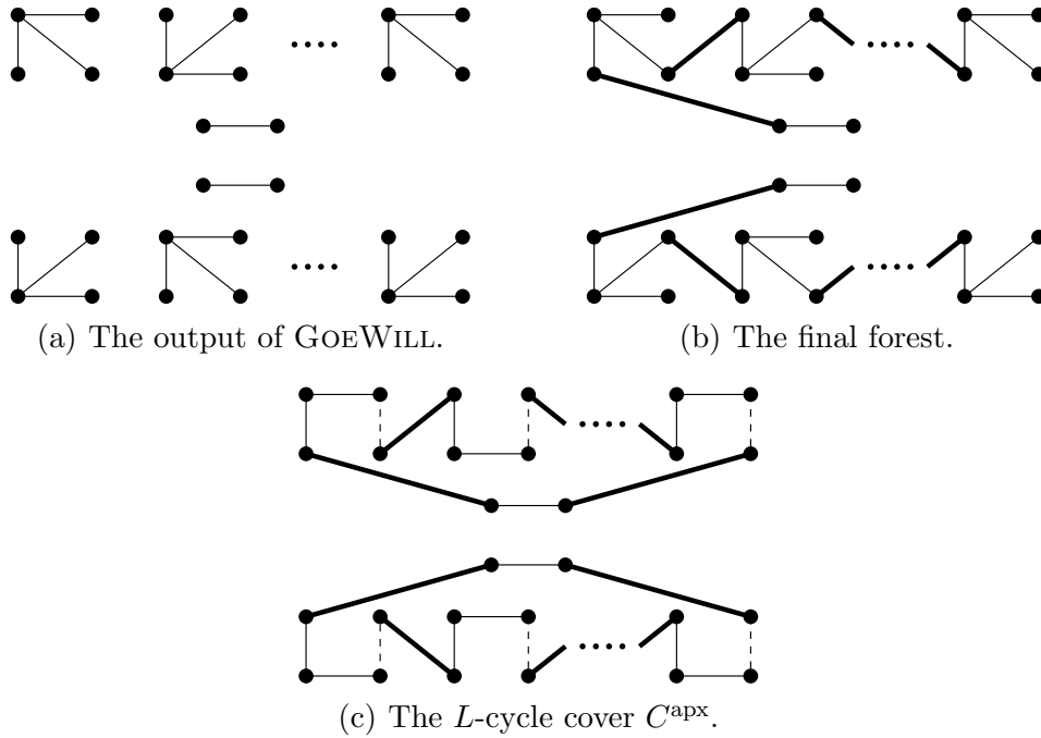
Fig. 2. How \text{APXUNDIR}_{L'} computes an L -cycle cover of the graph of Figure 1(a), even by these more general functions.
