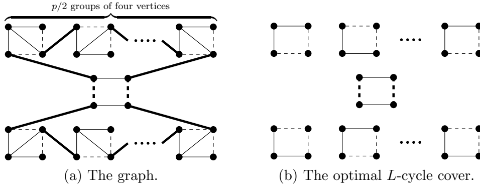
Fig. 1. An example on which \text{APXUNDIR}_{L'} achieves only a ratio of roughly p_L/2 .
